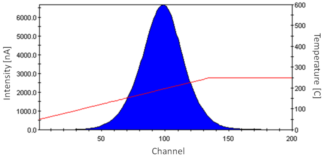
Figure 4-12: TL data for LTB: Ag irradiated with 5 keV electrons. A single peak at 196°C is observed.
