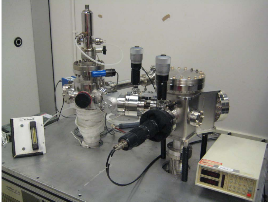
Figure 3-1: The VUV cathodoluminescence system in the CL lab at building 644. This system is unique in that light emitted from the sample travels through vacuum all the way until it is detected by the PMT. Therefore, high energy photons generally attenuated by the atmosphere or windows can be detected with this system.
